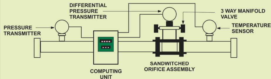
FIG : SCHEMATIC ARRANGEMENT FOR GFMc - 150
